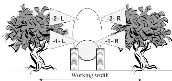
Figure 2-1: Airblast (AB) principle
