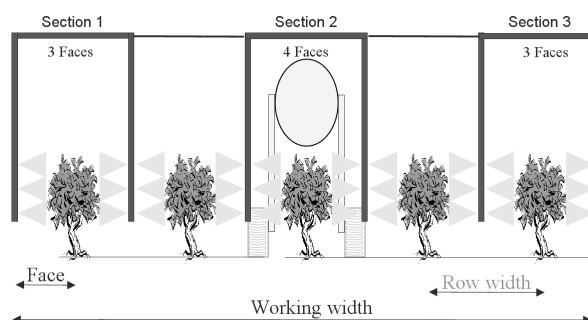
Figure 2-2: Airblast (AB) principle
