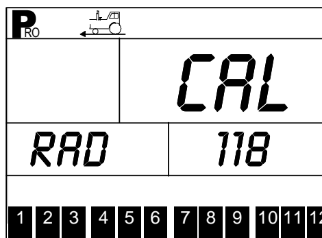
Figure 4-17: Radar Speed Sensor Automatic Calibration
