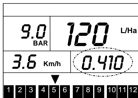
Figure 9-2: Area/Volume Display
