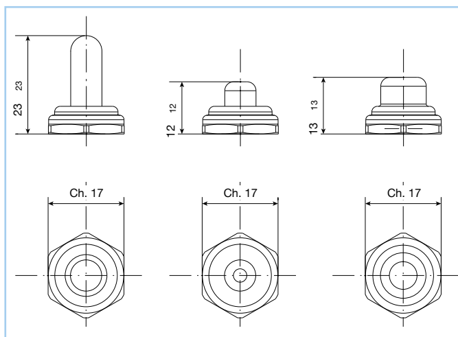
NYLON version OPTIONAL
